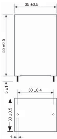
Specifications casing 1: Bucket: Plastic bucket UL 94-V0 Terminals: copper wire, tin-plated Ø1.4 mm Weight: approx. 70g
